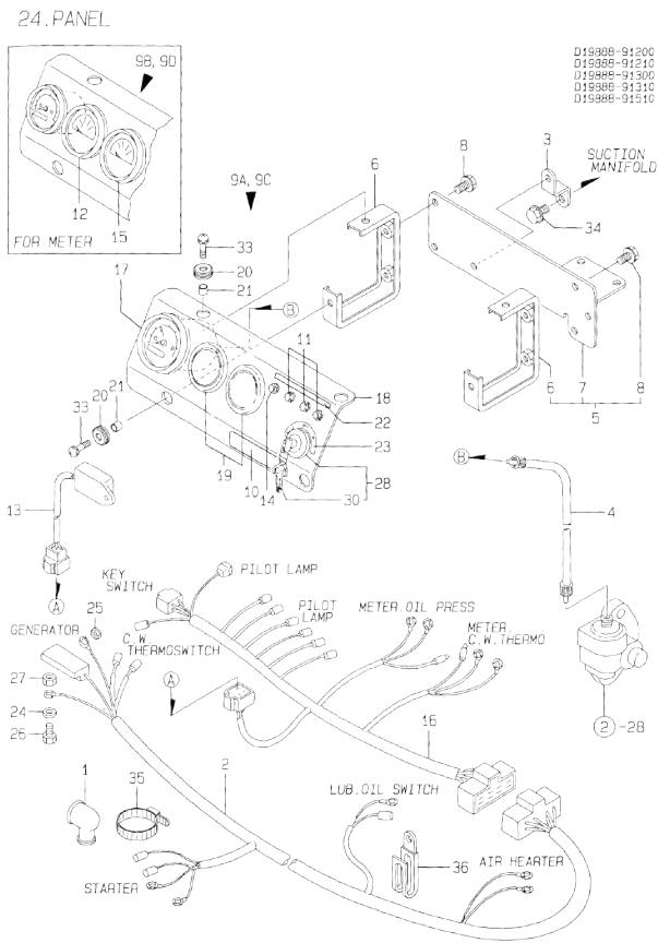
Fig.24. PANEL
