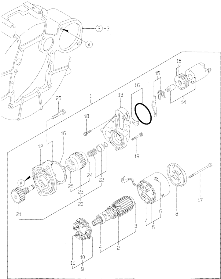
Fig.19. STARTING MOTOR(STANDARD)
